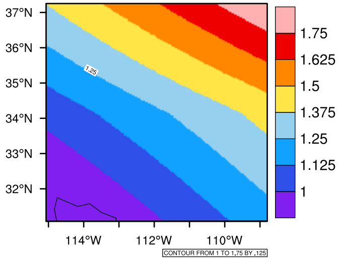
Yearly pr (mm/day) In 2020-2029 GFDL-ESM2M RCP45 - Arizona
