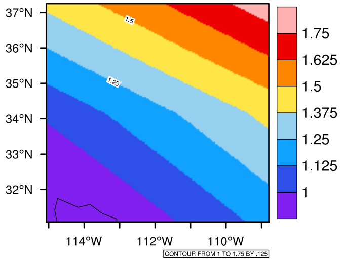
Yearly pr (mm/day) In 2020-2029 GFDL-ESM2M RCP85 - Arizona
