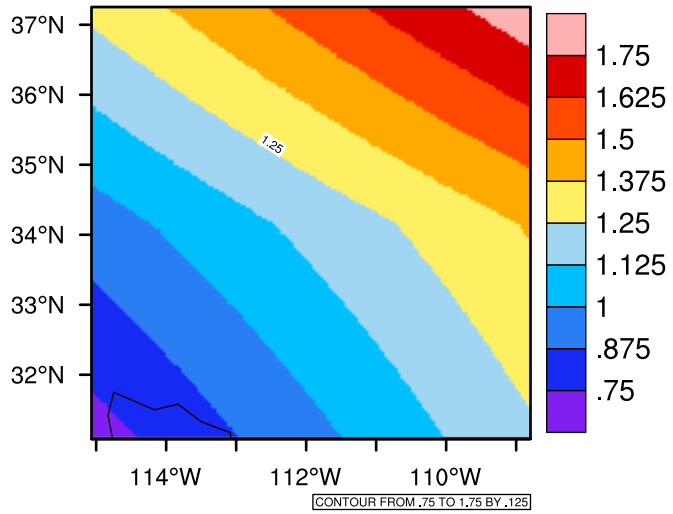
Yearly pr (mm/day) In 2040-2049 GFDL-ESM2M RCP85 - Arizona
