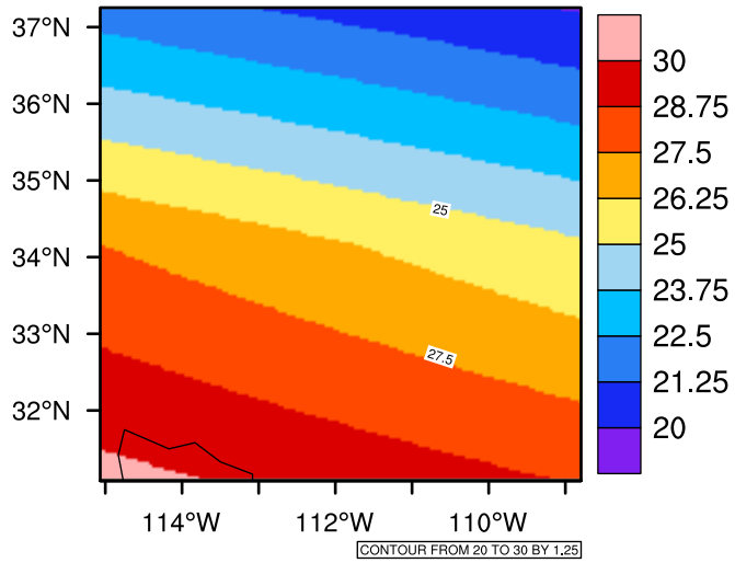
Yearly tasmax(c) In 2070-2079 GFDL-ESM2M RCP85 - Arizona
