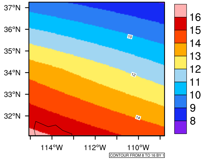
Yearly tasmin(c) In 2050-2059 GFDL-ESM2M RCP45 - Arizona
