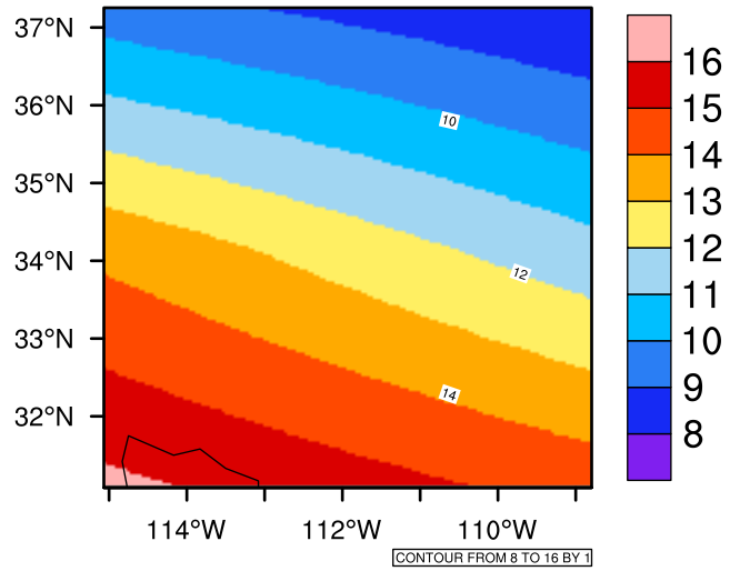
Yearly tasmin(c) In 2080-2089 GFDL-ESM2M RCP45 - Arizona
