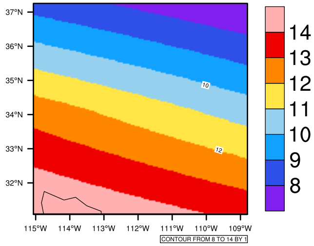
Yearly tasmin(c) In 1975-2005 GFDL-ESM2M historical - Arizona
