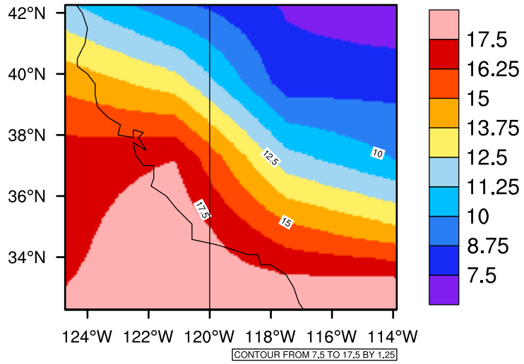
Yearly tas(c) In 2040-2049 GFDL-ESM2M RCP85 - California
