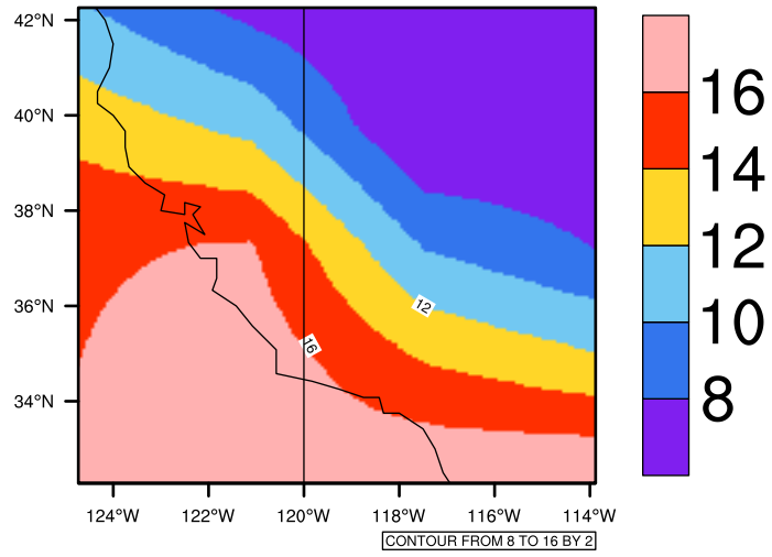
Yearly tas(c) in 1975-2005 GFDL-ESM2M historical - California
