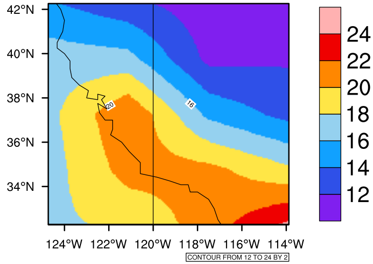
Yearly tasmax(c) In 2020-2029 GFDL-ESM2M RCP45 - California
