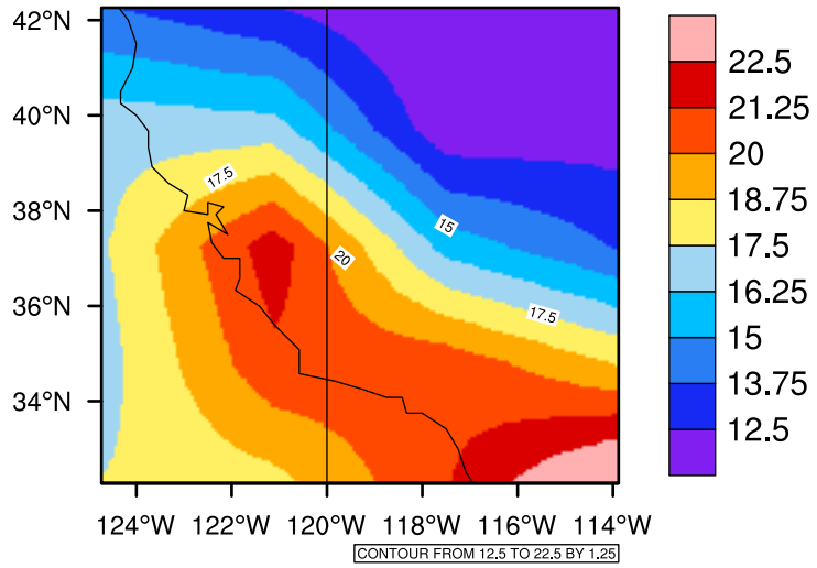
Yearly tasmax(c) In 2040-2049 GFDL-ESM2M RCP45 - California
