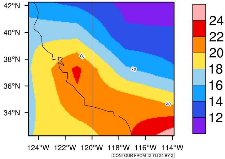
Yearly tasmax(c) In 2080-2089 GFDL-ESM2M RCP45 - California
