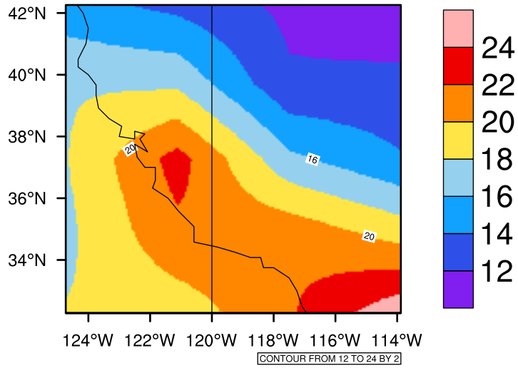
Yearly tasmax(c) In 2090-2099 GFDL-ESM2M RCP45 - California
