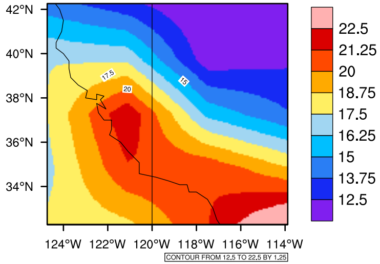
Yearly tasmax(c) In 2030-2039 GFDL-ESM2M RCP85 - California
