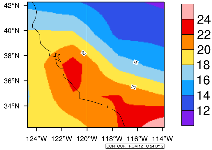
Yearly tasmax(c) In 2050-2059 GFDL-ESM2M RCP85 - California
