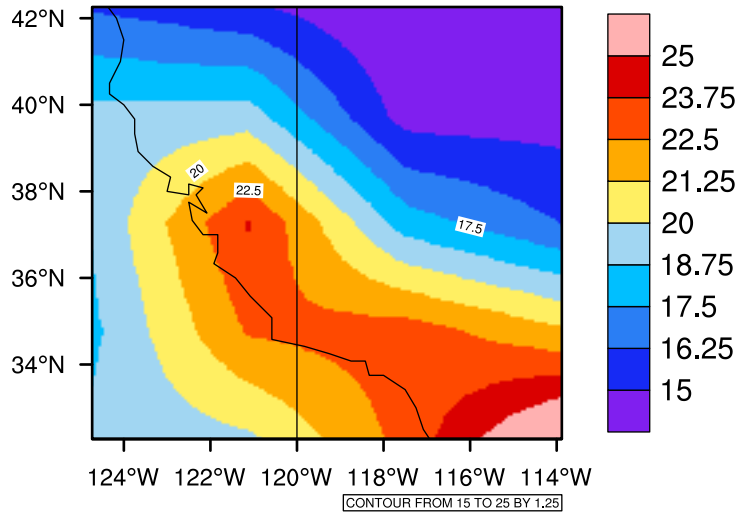
Yearly tasmax(c) In 2070-2079 GFDL-ESM2M RCP85 - California
