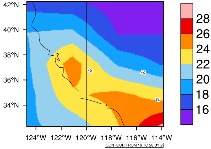
Yearly tasmax(c) In 2090-2099 GFDL-ESM2M RCP85 - California
