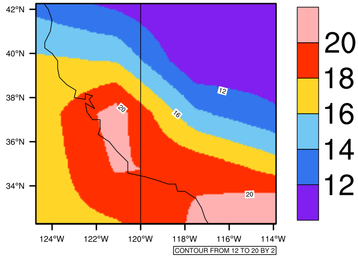
Yearly tasm max (c) in 1975-2005 GFDL-ESM2M historical - California
