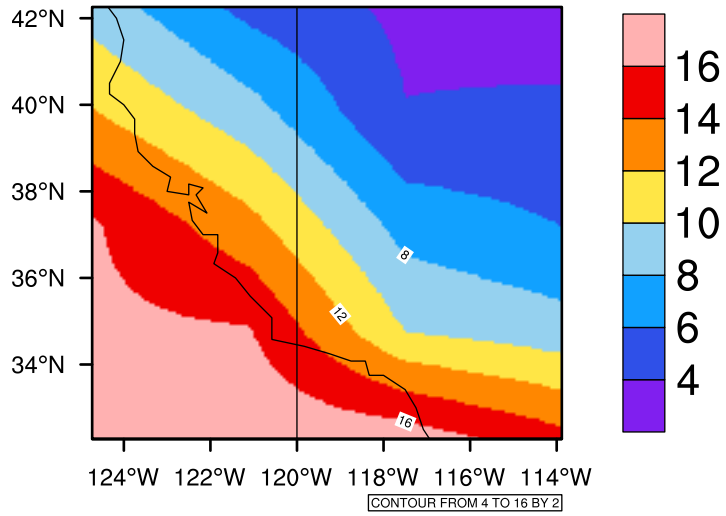
Yearly tasmin(c) In 2060-2069 GFDL-ESM2M RCP45 - California
