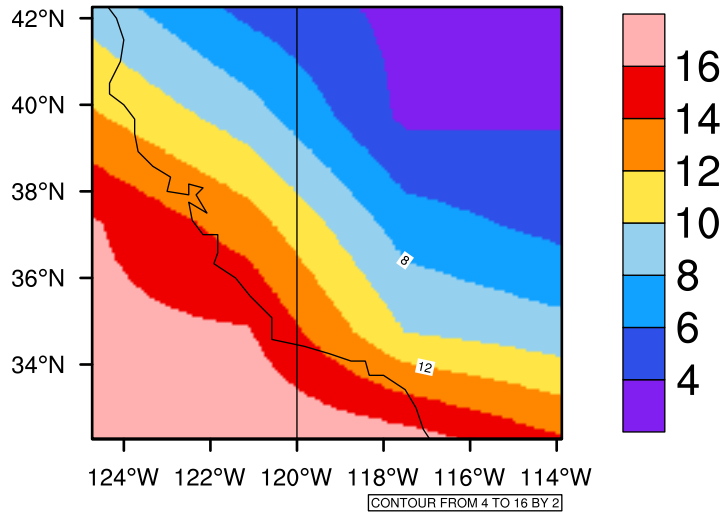
Yearly tasmin(c) In 2020-2029 GFDL-ESM2M RCP85 - California
