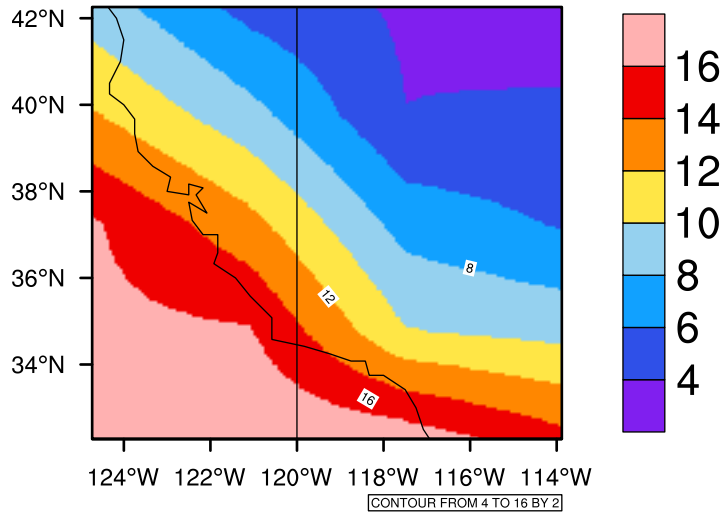
Yearly tasmin(c) In 2040-2049 GFDL-ESM2M RCP85 - California
