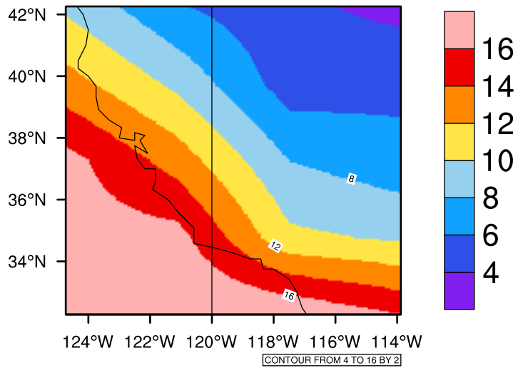
Yearly tasmin(c) In 2060-2069 GFDL-ESM2M RCP85 - California
