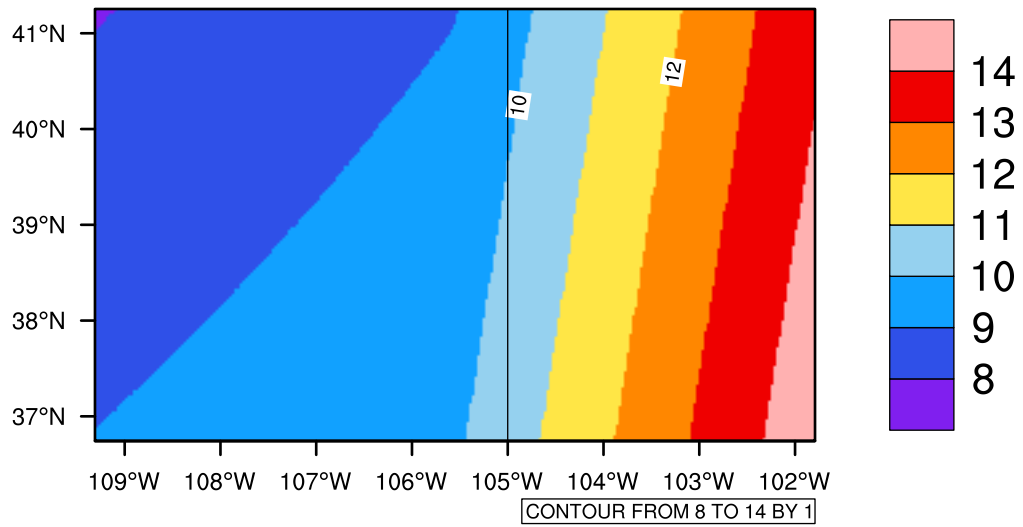
Yearly tasmax(c) In 2030-2039 GFDL-ESM2M RCP85 - Colorado
