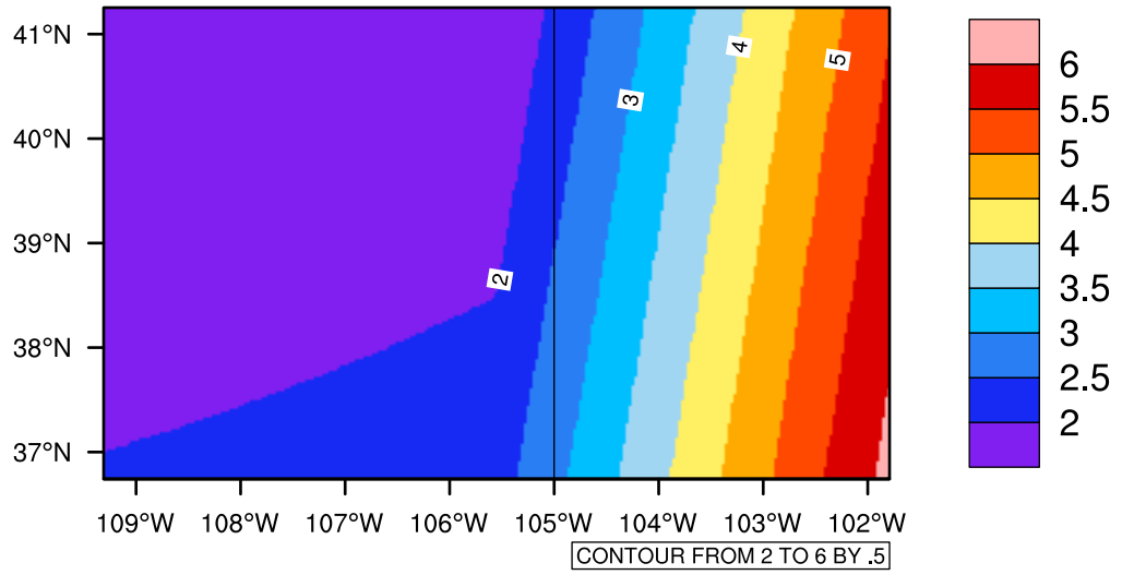
Yearly tasmin(c) In 2050-2059 GFDL-ESM2M RCP85 - Colorado
