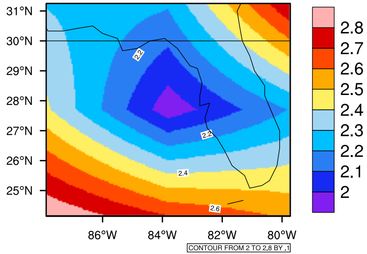
Yearly pr (mm/day) In 2020-2029 GFDL-ESM2M RCP45 - Florida
