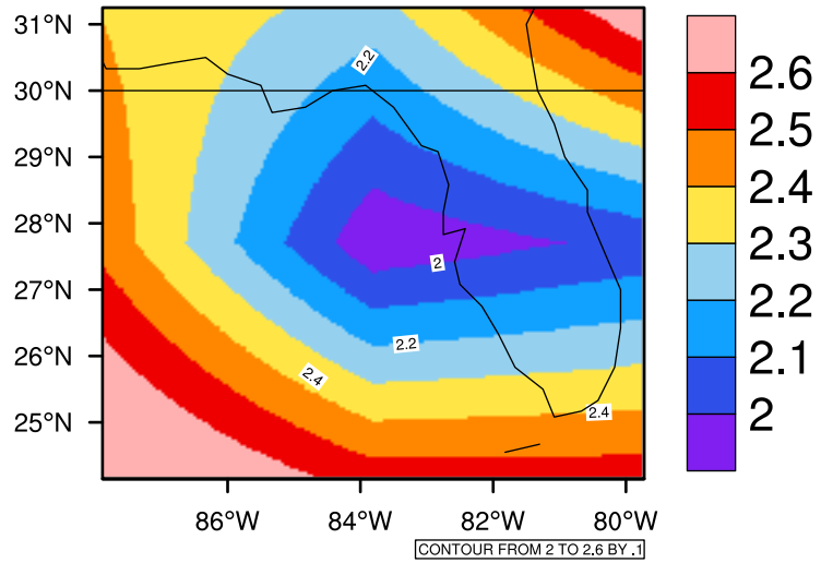
Yearly pr (mm/day) In 2030-2039 GFDL-ESM2M RCP45 - Florida
