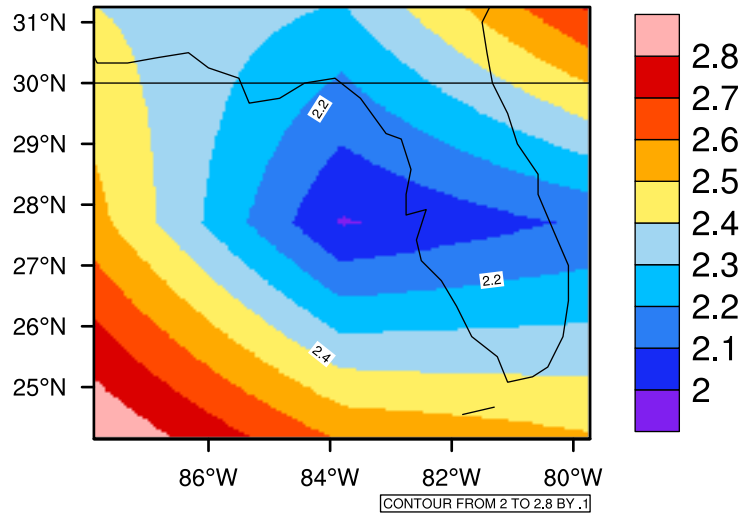
Yearly pr (mm/day) In 2050-2059 GFDL-ESM2M RCP45 - Florida
