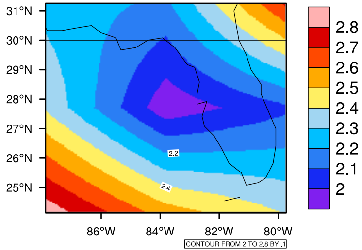
Yearly pr (mm/day) In 2060-2069 GFDL-ESM2M RCP45 - Florida
