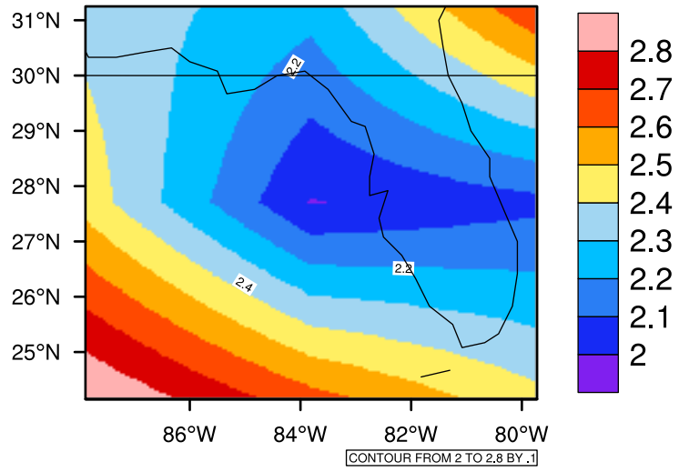
Yearly pr (mm/day) In 2070-2079 GFDL-ESM2M RCP45 - Florida
