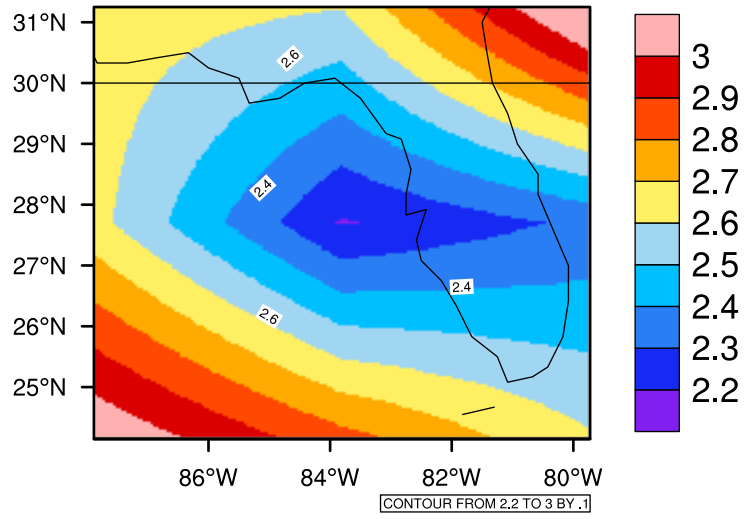
Yearly pr (mm/day) In 2080-2089 GFDL-ESM2M RCP45 - Florida
