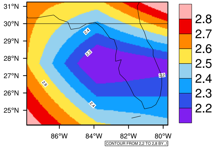
Yearly pr (mm/day) In 2040-2049 GFDL-ESM2M RCP85 - Florida
