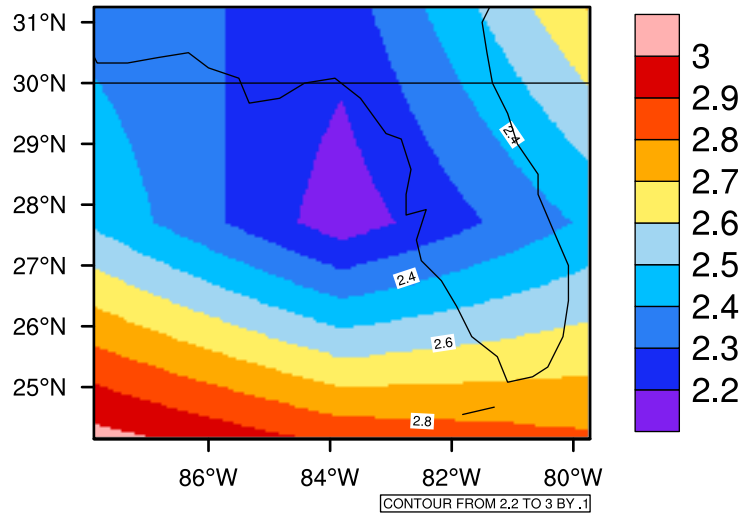
Yearly pr (mm/day) In 2050-2059 GFDL-ESM2M RCP85 - Florida
