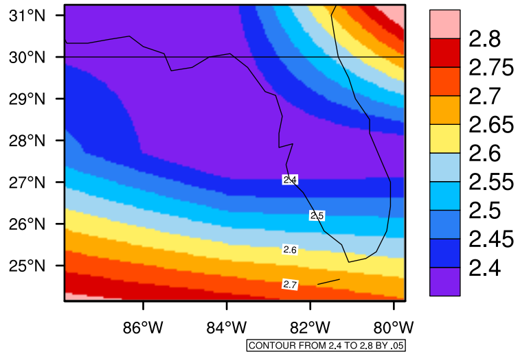
Yearly pr (mm/day) In 2070-2079 GFDL-ESM2M RCP85 - Florida
