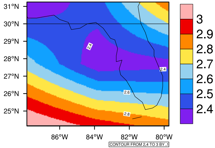
Yearly pr (mm/day) In 2080-2089 GFDL-ESM2M RCP85 - Florida
