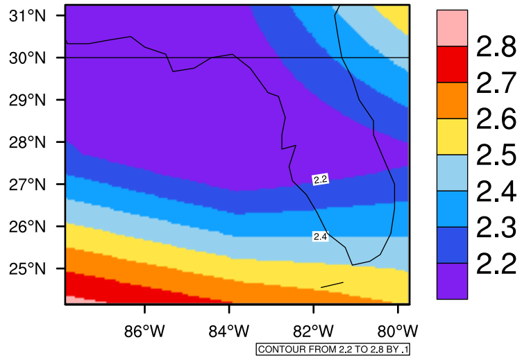
Yearly pr (mm/day) In 2090-2099 GFDL-ESM2M RCP85 - Florida
