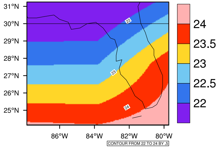
Yearly tas(c) In 2020-2029 GFDL-ESM2M RCP45 - Florida
