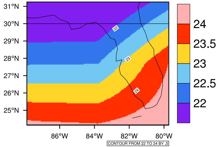
Yearly tas(c) In 2030-2039 GFDL-ESM2M RCP45 - Florida
