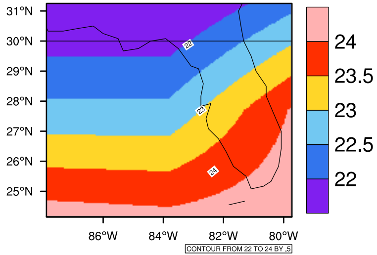
Yearly tas(c) In 2040-2049 GFDL-ESM2M RCP45 - Florida
