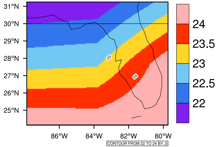
Yearly tas(c) In 2050-2059 GFDL-ESM2M RCP45 - Florida
