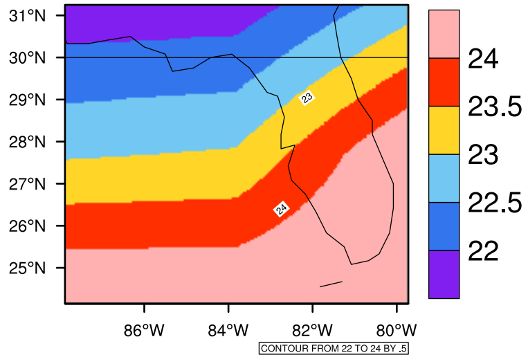
Yearly tas(c) In 2060-2069 GFDL-ESM2M RCP45 - Florida
