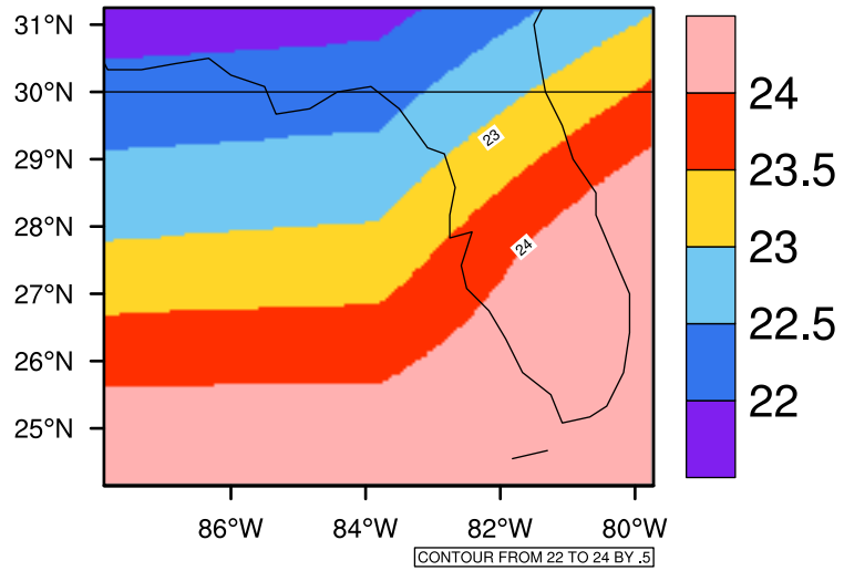
Yearly tas(c) In 2070-2079 GFDL-ESM2M RCP45 - Florida
