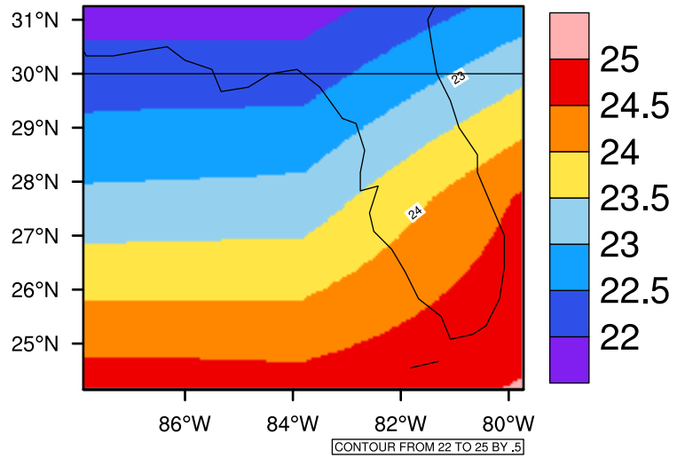
Yearly tas(c) In 2080-2089 GFDL-ESM2M RCP45 - Florida
