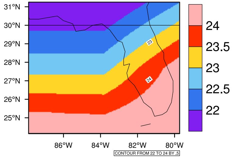
Yearly tas(c) In 2040-2049 GFDL-ESM2M RCP85 - Florida
