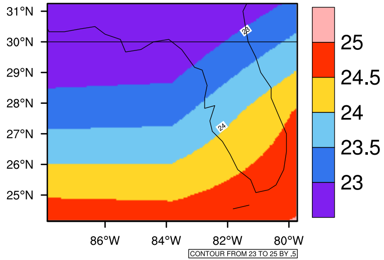
Yearly tas(c) In 2050-2059 GFDL-ESM2M RCP85 - Florida
