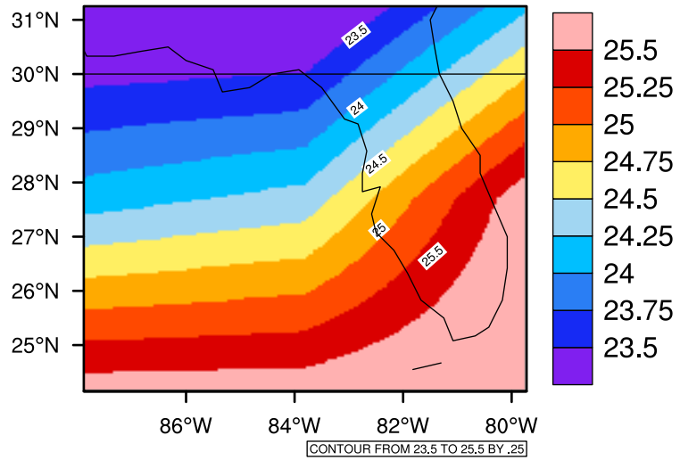
Yearly tas(c) In 2070-2079 GFDL-ESM2M RCP85 - Florida
