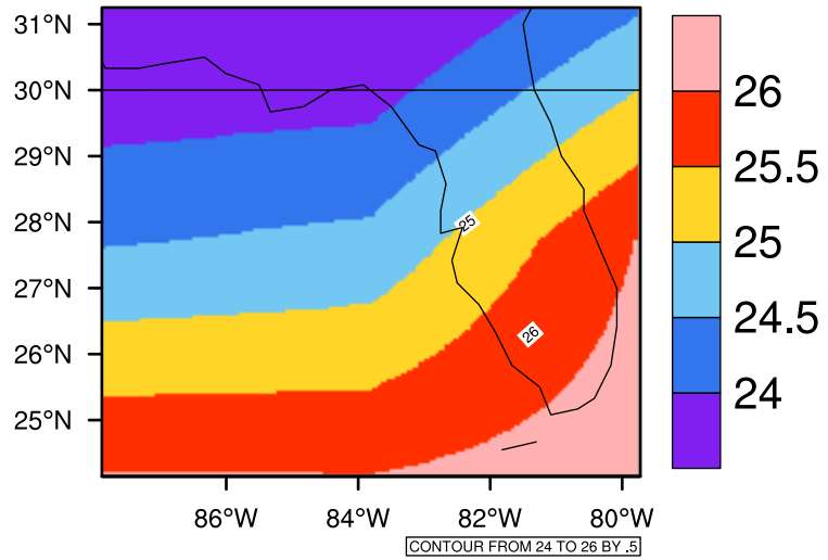
Yearly tas(c) In 2080-2089 GFDL-ESM2M RCP85 - Florida
