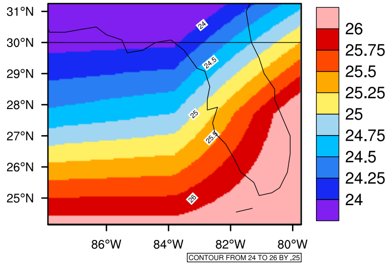
Yearly tas(c) In 2090-2099 GFDL-ESM2M RCP85 - Florida
