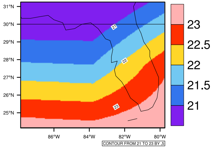
Yearly tas(c) In 1975-2005 GFDL-ESM2M historical - Florida
