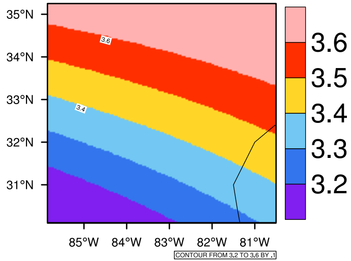
Yearly pr (mm/day) In 2020-2029 GFDL-ESM2M RCP45 - Georgia
