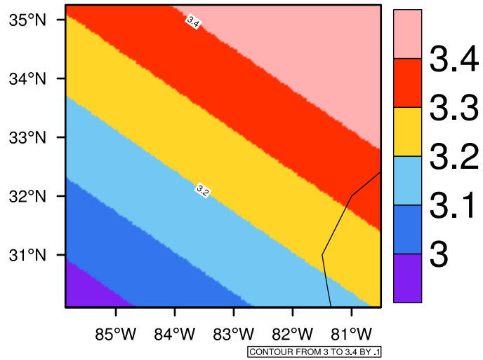
Yearly pr (mm/day) In 2030-2039 GFDL-ESM2M RCP45 - Georgia
